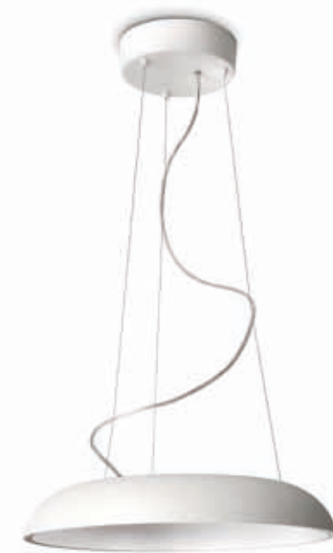
Amaze 40233/31/16 1 1400 → 434 ↗ 434 2GX13 - 1x 60W incl. - 5000 lm - 2700K ☹ - IP20 metal - synthetics
