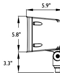
LPF2WG wire guard (field installed)
