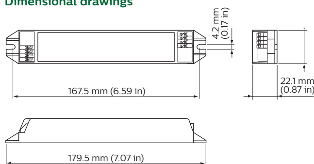
Controller LLC1663 dimensions
