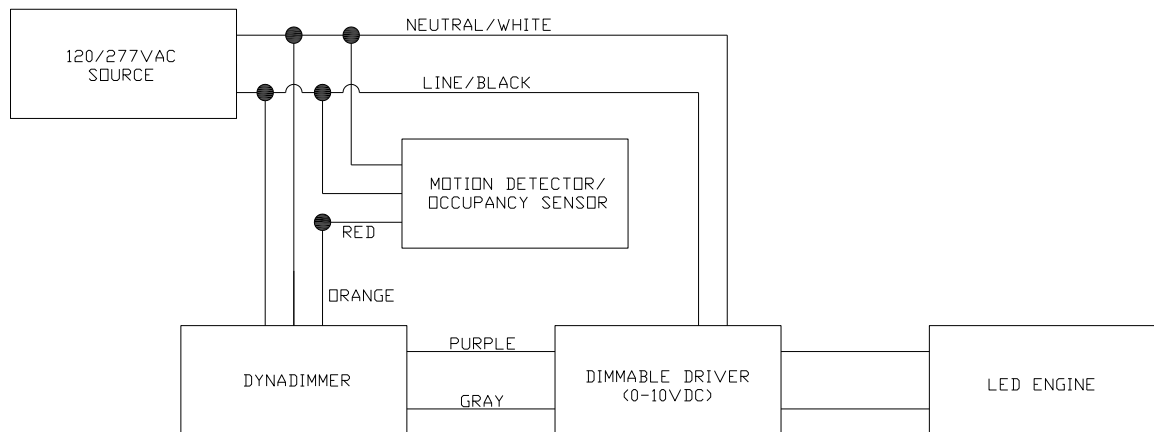
WIRE DIAGRAM FOR MRO WITH DYNADIMMER
