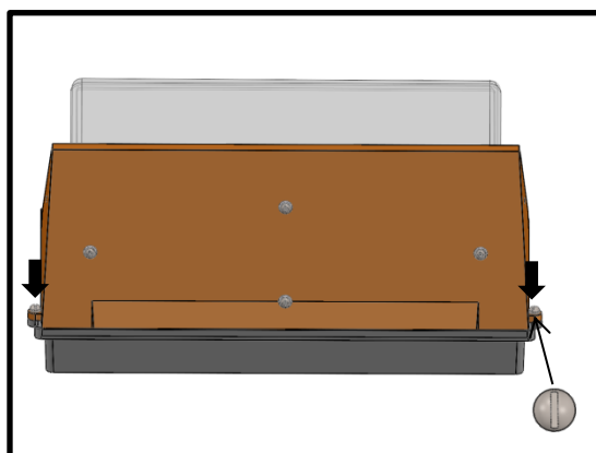
STEP 6: Close the lens frame and tighten the screws to fasten the lens frame to the housing.
