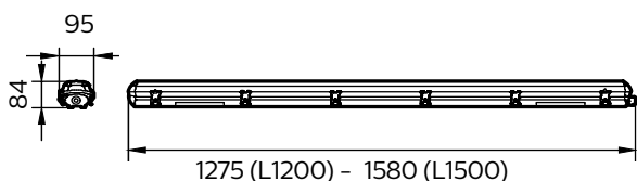
WT050C 2 Tubes
