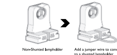
Figure showing how to convert a non-shunted lampholder to a shunted lamp holder using a jumper wire.
