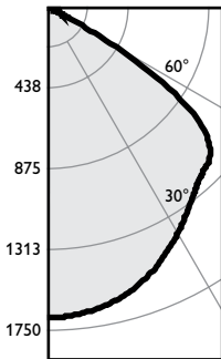
Candela Curve
