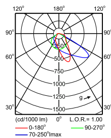
IFPS_4MX400 491 1xLED55S/830 PSD A20- Polar Normal (separate)
