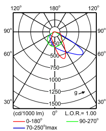
IFPS_4MX400 491 1xLED40S/830 PSD A20- Polar Normal (separate)
