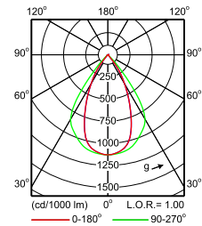
IFPS_4MX400 G3 581 1xLED80S/830 PSD NB- Polar Normal (separate)
