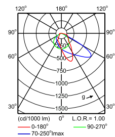
IFPS_4MX400 G2 491 1xLED55S/840 PSD A20- Polar Normal (separate)
