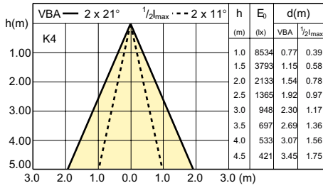
LDBE_CDM-R111_35W_24D-Beam diagram
