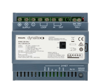
DDBC120-DALI MultiMaster DALI Driver Controller
