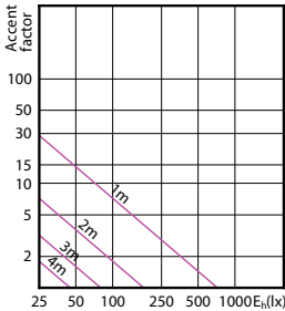
SceneSwitch LED Lamps 50W GU10 827 36D SSW
