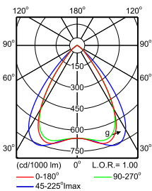
IFPS_DN572B PSE-E 1xLED24S/830 C-Polar Normal (separate)
