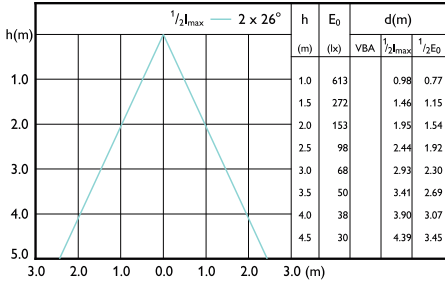
Beam diagram - MAS LED MR16 ExpertColor 6.7-50W 940 60D
