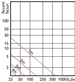
Accent Diagram - MAS LED MR16 ExpertColor 6.7-50W 940 60D
