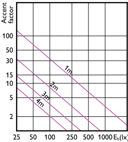
Accent Diagram - MASTER LED 7.5-50W+ 830 MR16 24D Dim
