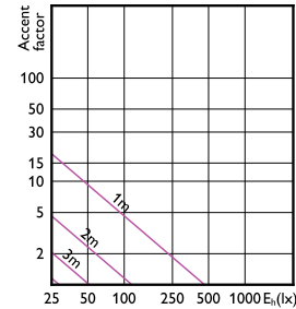
Accent Diagram - MASTER LED 6.5-50W 930 MR16 60D Dim
