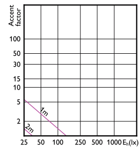
Accent Diagram - CoreProLEDspot ND1.8-30W R39 E14 827 36D
