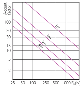
Accent Diagram - Master LED PAR30L 32W 15D 830
