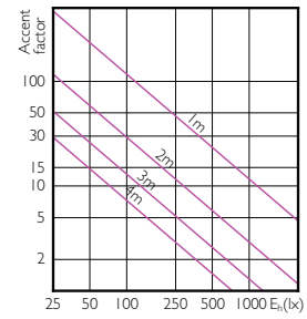
Accent Diagram - Master LED PAR30L 32W 30D 830
