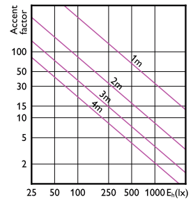
Accent Diagram - Master LED PAR30L 28W 15D 830 100-277V
