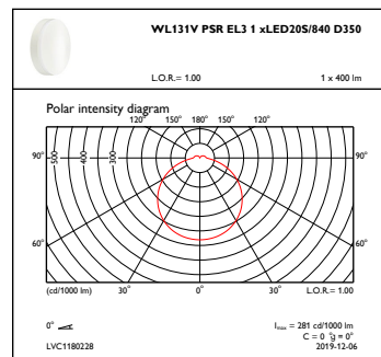
OFPC1_WL131VPSREL31xLED20S840D350
