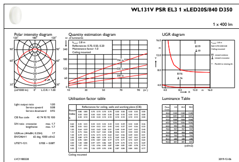
IFGU1_WL131VPSREL31xLED20S840D350
