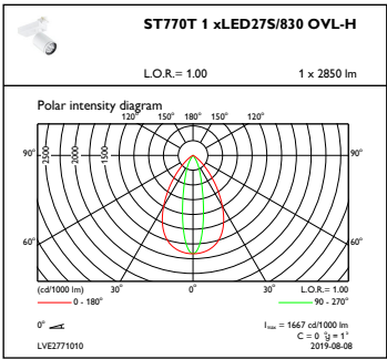
OFPC1_ST770T1xLED27S830OVL-H
