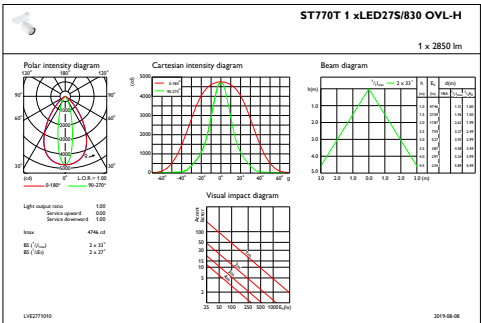
IFAS1_ST770T1xLED27S830OVL-H
