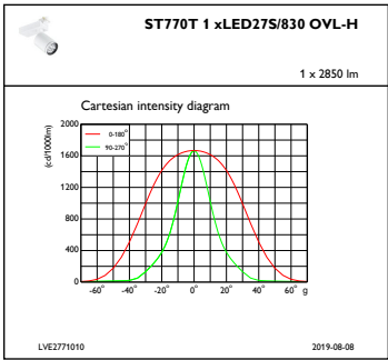
IFCC1_ST770T1xLED27S830OVL-H
