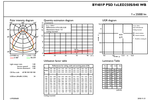
IFGU1_BY481PPSD1xLED250S840WB
