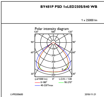
IFPC1_BY481PPSD1xLED250S840WB
