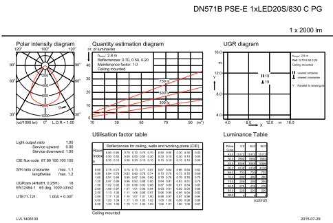
IFGU1_DN571B PSE-E 1xLED20S830 C PG.EPS
