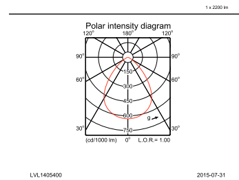
DN570B PSED-E 1xLED20S/830 C
