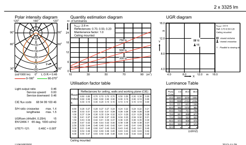
TCS461 2xTL5-35W HFP AC-MLO
