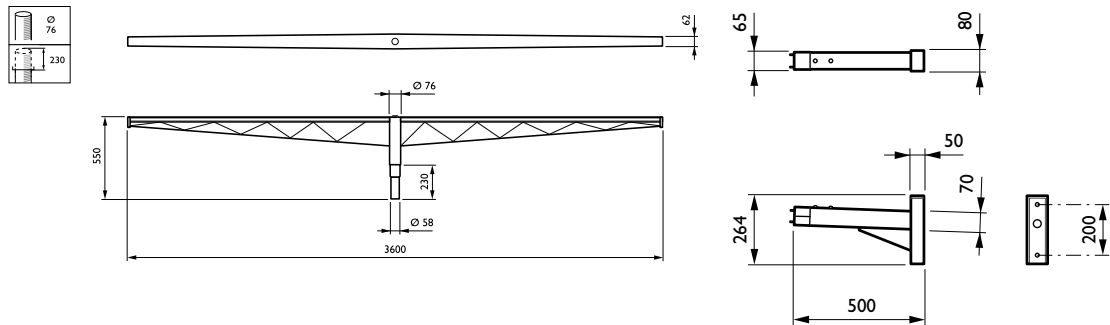
CitySoul gen2 brackets JGP530-JRP534
