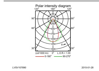
IFPC_4MX400 G3 491 1xLED40S/840 PSD NB-Polar Indoor (combined)
