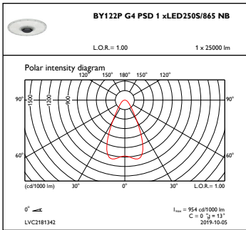
OFPC1_BY122PG4PSD1xLED250S865NB
