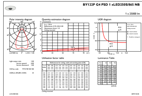
IFGU1_BY122PG4PSD1xLED250S865NB
