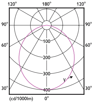
Light Distribution Diagram - DN027B LED6/CW D90 RD
