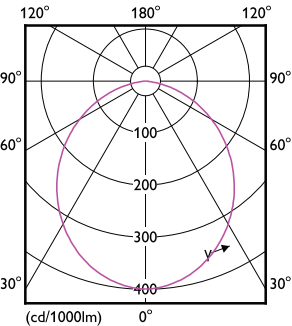
Light Distribution Diagram - DN027B LED9/CW D150 RD
