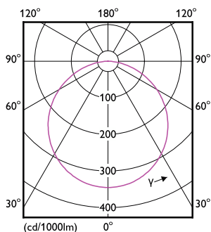
Light Distribution Diagram - DN027B LED9/CW L150 SQ
