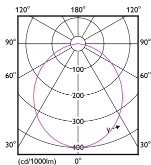
Light Distribution Diagram - DN027C LED9/NW D150
