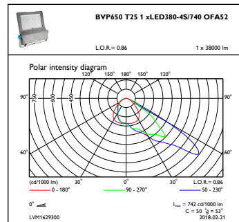
OFPC1_BVP650T251xLED380-4S740OFA52
