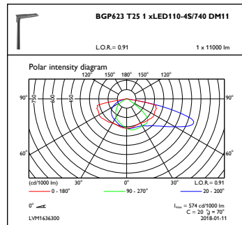
OFPC1_BGP623T251xLED110-4S740DM11
