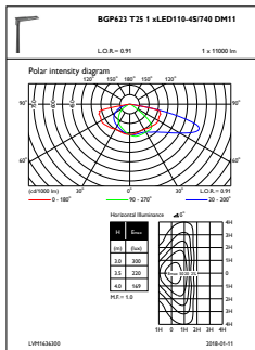
OFPL1_BGP623T251xLED110-4S740DM11
