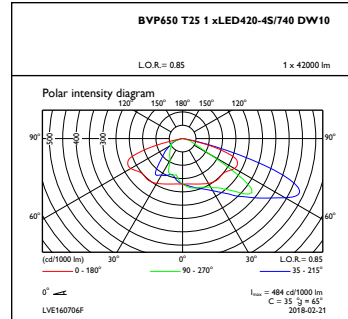
OFPC1_BVP650T251xLED420-4S740DW10
