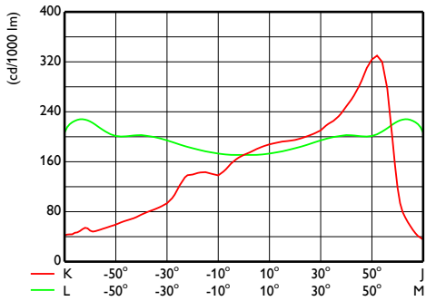
OFCS1_BVP650T251xLED420-4S740DW10
