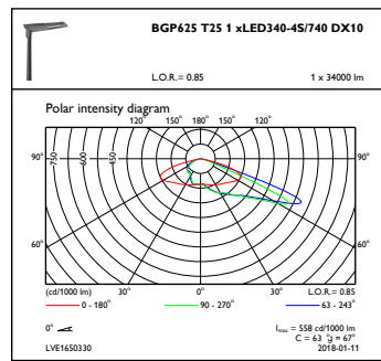
OFPC1_BGP625T251xLED340-4S740DX10
