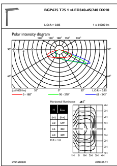
OFPL1_BGP625T251xLED340-4S740DX10
