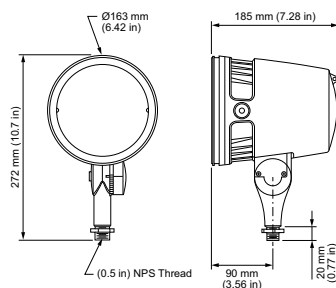
BCP463 G2 19xLED-HB/2700 HMA BZ
