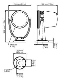
BCP463 G2 19xLED-HB/4000 WH
