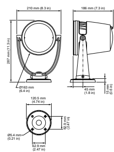
BCP463 G2 19xLED-HB/3000 BZ
