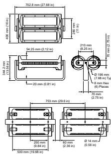
DCP773 72xLED-HB/2700K
