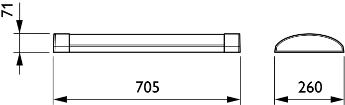
Dimensional drawing
