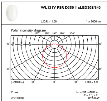
OFPC1_WL131VPSRD3501xLED20S840
