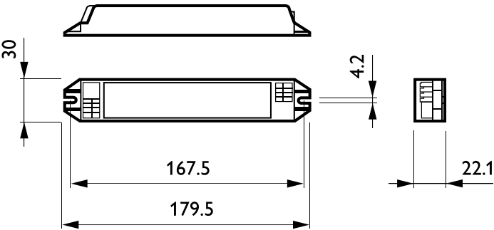
Dimensional drawing
