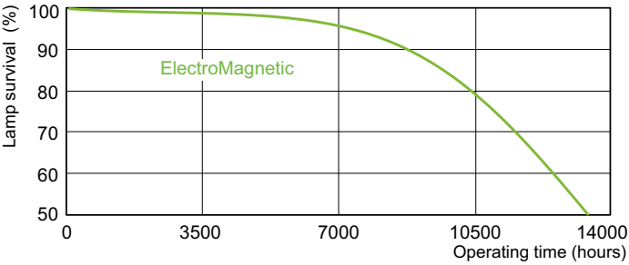
Life Expectancy Diagram - PL-S 13W/841/2P 1CT/5X10BOX ALTO
