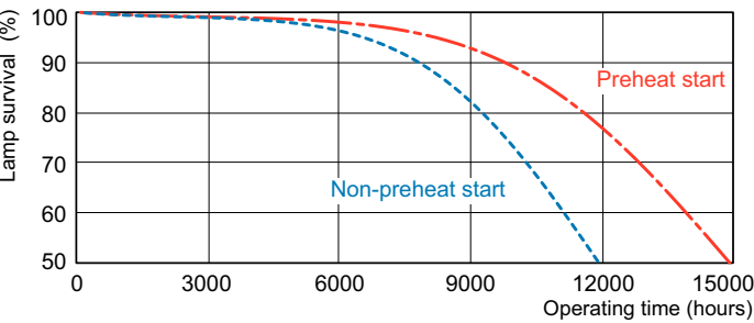
Life Expectancy Diagram - PL-C 18W/827/4P/ALTO 10PK
