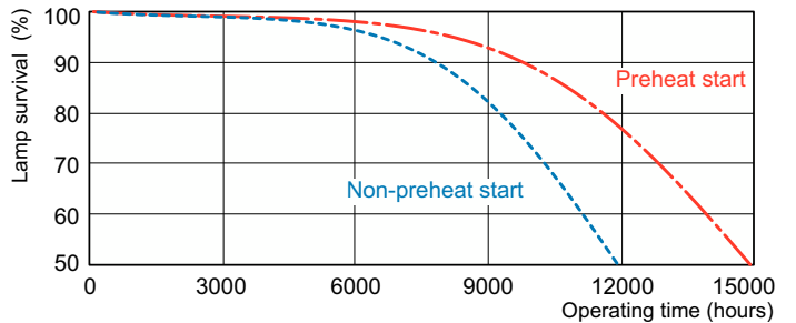
Life Expectancy Diagram - MASTER PL-C 26W/830/4P 1CT/5X10BOX
