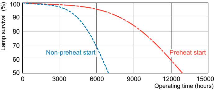
Life Expectancy Diagram - PL-T 32W/830/A/4P 1CT/5X10BOX ALTO
