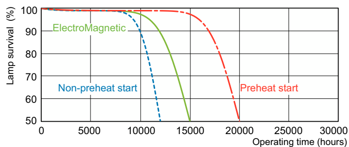
Life Expectancy Diagram - TL-D 30W/840 1PP/10
