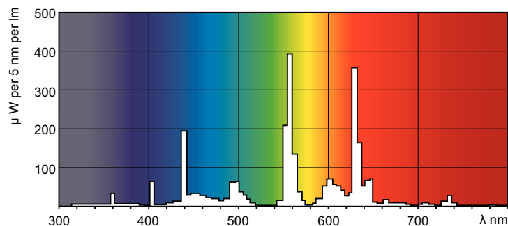
Spectral Power Distribution Colour - TL-D 30W/840 1PP/10
