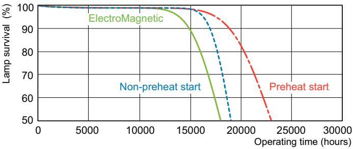
Life Expectancy Diagram - TL-D 15W/827 1PP/10
