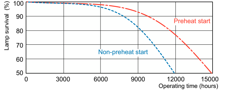
Life Expectancy Diagram - MASTER PL-S 9W/840/4P 1CT/5X10BOX
