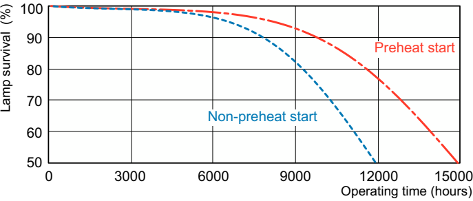
Life Expectancy Diagram - MASTER PL-S 11W/840/4P 1CT/10
