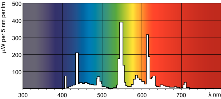
Spectral Power Distribution Colour - MASTER PL-S 11W/840/4P 1CT/10
