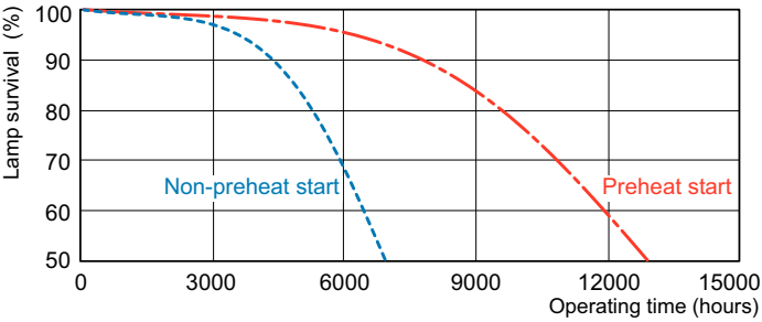
Life Expectancy Diagram - MASTER PL-S 11W/840/4P 1CT/10
