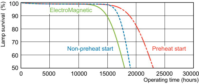
Life Expectancy Diagram - TL-D 36W/827 1SL/25
